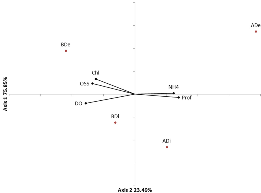
Figure 4. Correspondence Canonical Analysis (CCA) between environmental- Chlorophyll (Chl), Organics suspended solids (OSS), dissolved oxygen (DO), Profundity (Prof) and ammonia (NH4) and biological variables- Archaeal density (ADe) Bacterial density (BDe), Archaeal diversity (ADi) and Bacterial diversity (BDi) from Itupararanga Reservoir, SP, Brazil.
