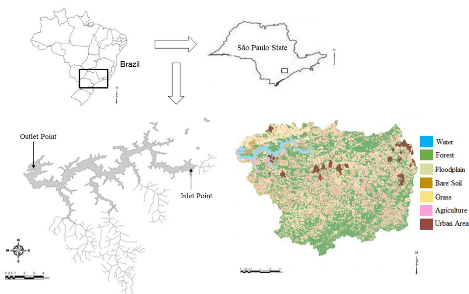
Figure 1. Location of São Paulo State in Brazil, Itupararanga Reservoir with the main tributaries and sampling points arrowed (Inlet Point: Headwater; Outlet Point: Dam) and the land use of Itupararanga basin.
