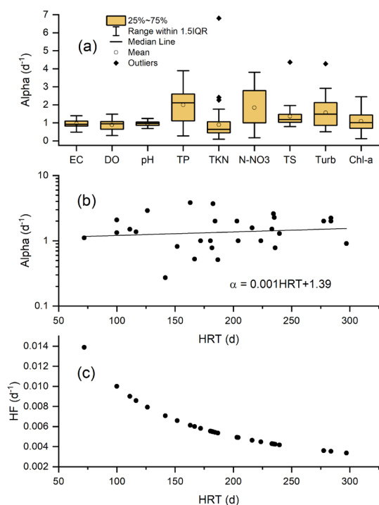
Figure 5. Alfa values for different water variables (a). Relationships between hydraulic retention time (HRT) of the Ituparanga Reservoir, and the retention capability ( \alpha ) for total phosphorus (b), hydraulic flows (HF) (c).
