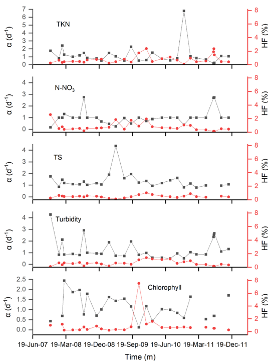
Figure 4. Total Kjeldhal nitrogen (TKN), nitrate (in N basis; N-NO 3 ), total solids (TS), turbidity, and chlorophyll- a retention parameters ( \alpha ; black line and square), and hydraulic flows (HF; red line and circle) in terms of \alpha percentage.
