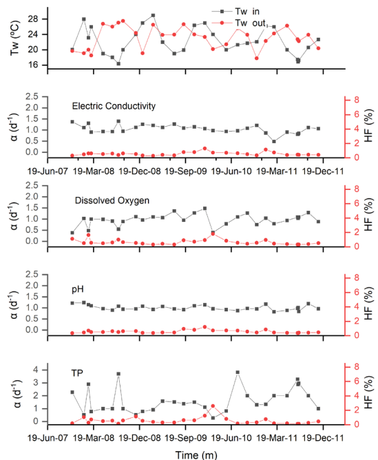
Figure 3. Water temperature changes in inlet and outlet sites of reservoir. Electric Conductivity, dissolved oxygen, pH, and Total Phosphorous (TP) retention parameters ( \alpha ; black line and square), and hydraulic flows (HF; red line and circle) in terms of \alpha percentage.
