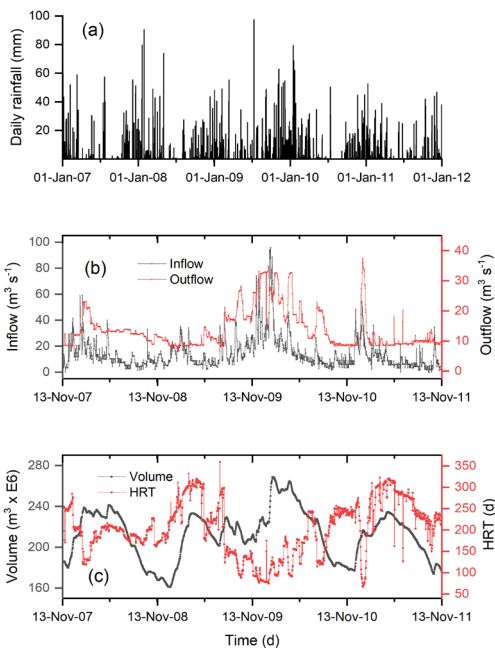
Figure 2. Daily rainfall in the dam area of Itupararanga Reservoir (a). Hydraulic characteristics of Itupararanga Reservoir: Flow data (b), and volume and Hydraulic Retention Time (HRT) (c); (Bottino, 2011; Casali, 2014; Votorantim Energia weather station: 23^\circ 36' 43.35''\text{S} ; 47^\circ 23' 49.87''\text{W} ).
