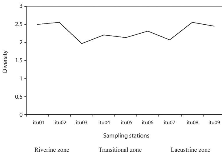
Fig. 6. Shannon diversity index for the Itupararanga Reservoir, using numeric abundance.
